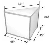
Pakyla (trikampė) Triangular platform
